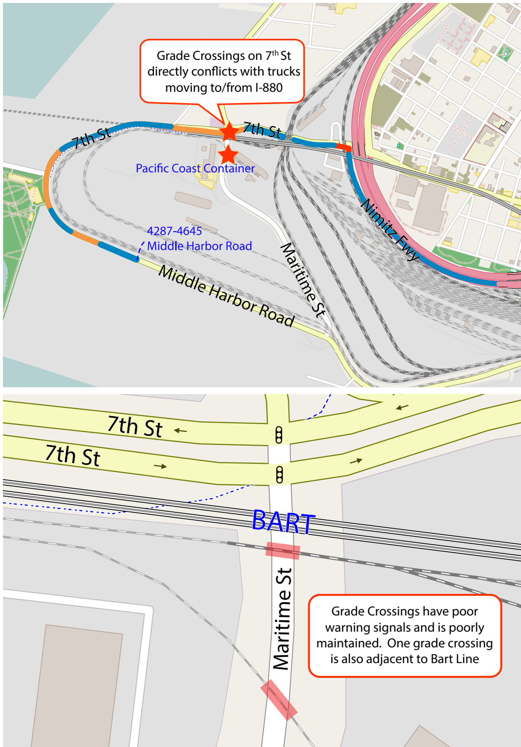
Figure 5.2 Grade Crossings at 7 th Street and Connectivity to I-880
