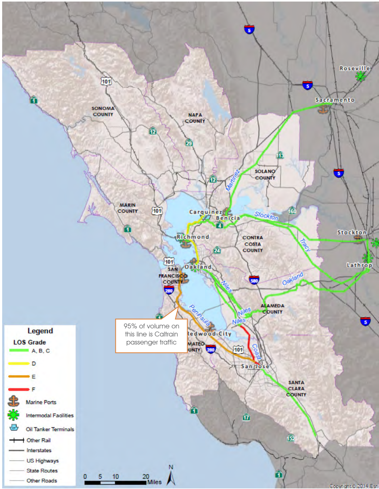
Figure 5.5 Bay Area Rail Existing LOS
