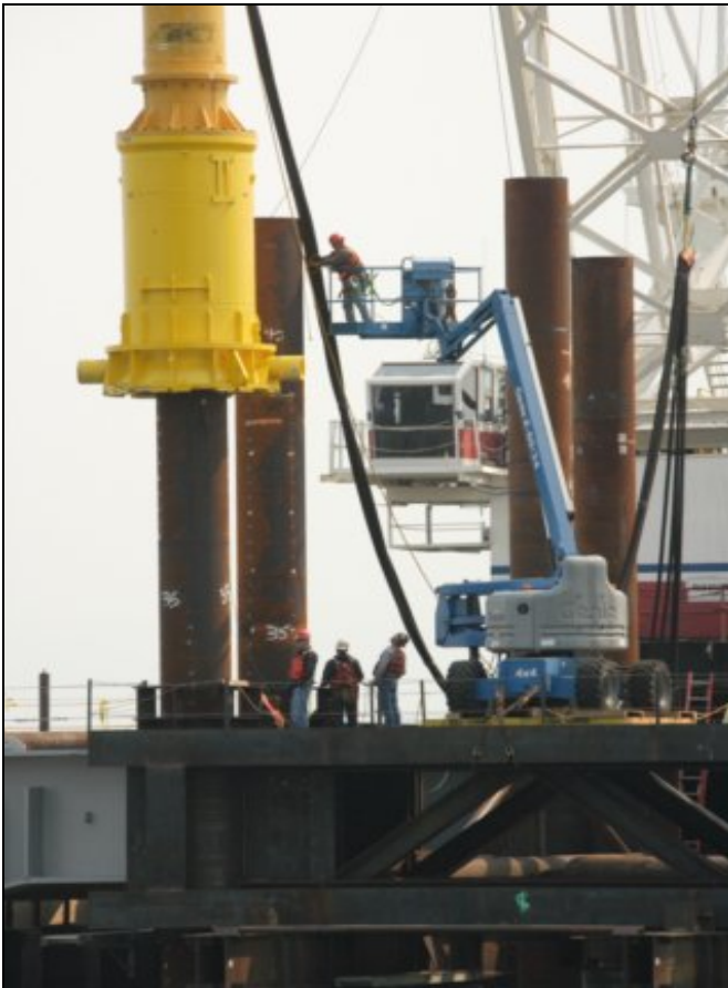
Temporary Tower D Pile Driving
