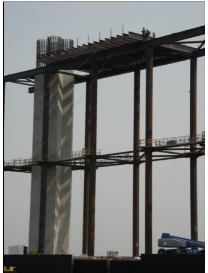
E2 – Temporary Falsework around E2
